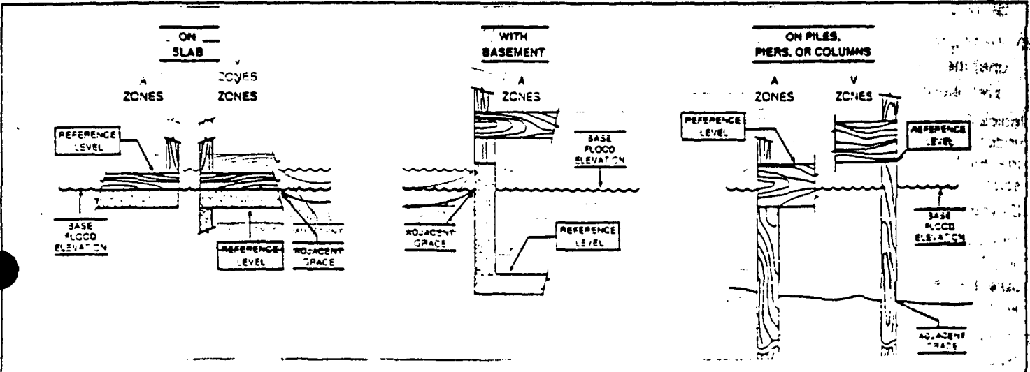
The diagrams above illustrate the points at which the elevations should be measured in A Zones and V Zones. Elevations for all A Zones should be measured at the top of the reference level floor.
